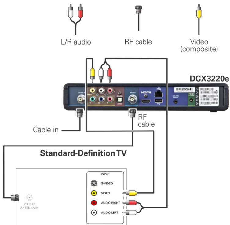
Figure 7: Connecting an SDTV
