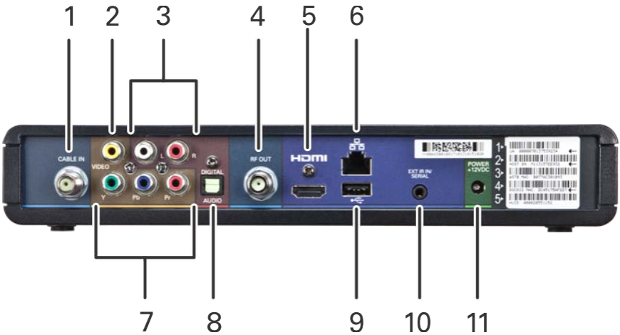
Figure 2: Rear Panel
