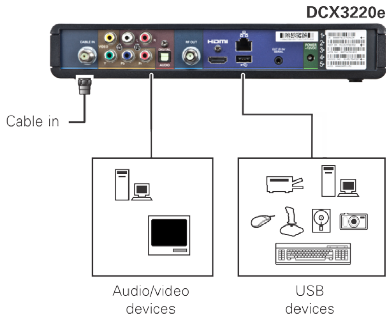
Figure 10: Data Device connections
