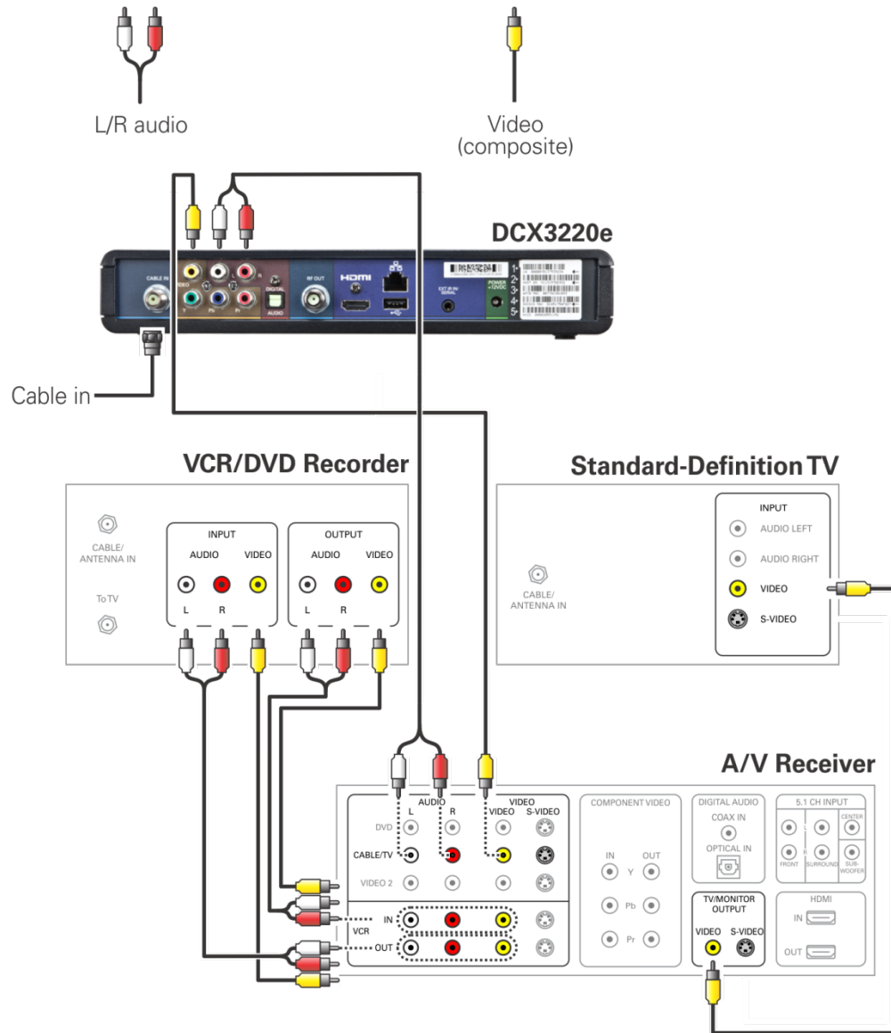
Figure 9: Connecting an A/V Receiver, SDTV, and VCR/DVD Recorder
