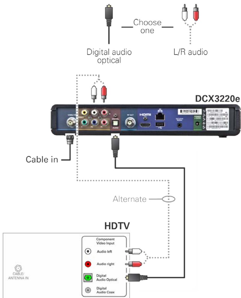
Figure 5: Connecting to an HDTV — Alternate Audio Connections
