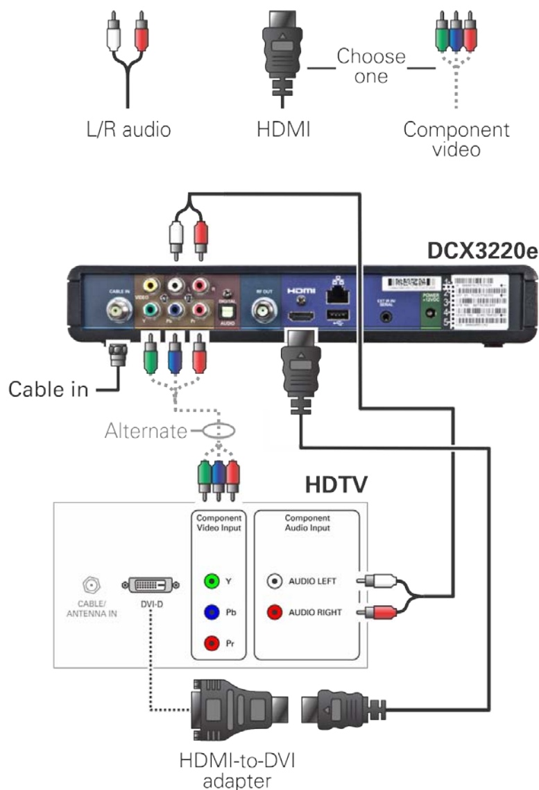
Figure 4: Connecting an HDTV — Separate Video/Audio Connections
