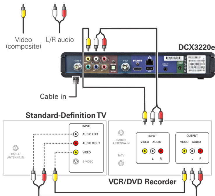
Figure 8: Connecting an SDTV and VCR/DVD Recorder
