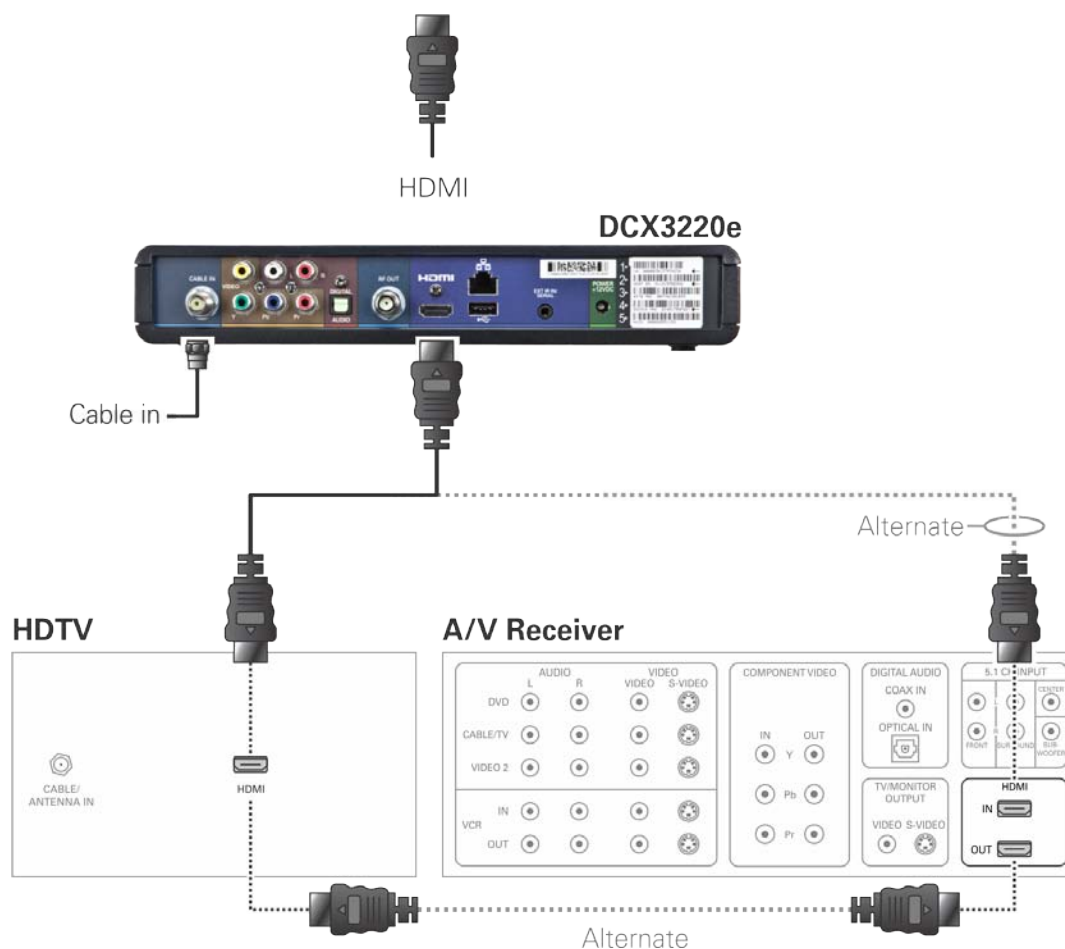
Figure 3: Connecting an HDTV — Single Connection for Video/Audio
