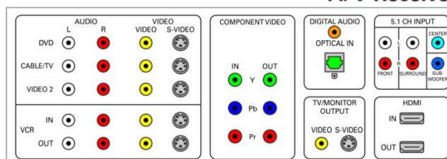
A/V Receiver
